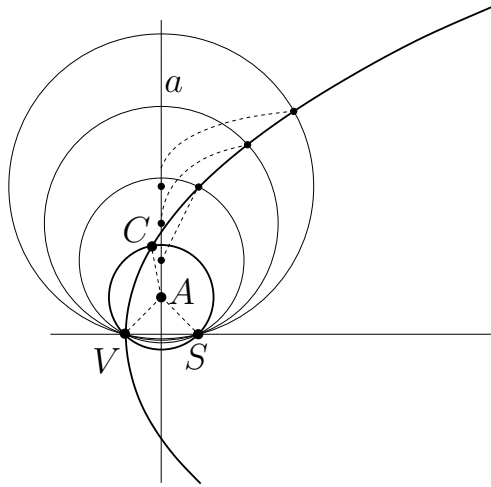
Fig. 6. The motion of the comet on a parabolic orbit.
