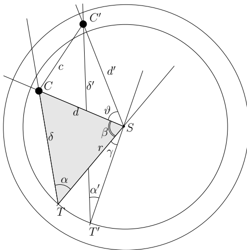
Fig. 2. Using the second observation and the uniformity of the motion on the chord the distance \delta' can be calculated as a function of \delta .
