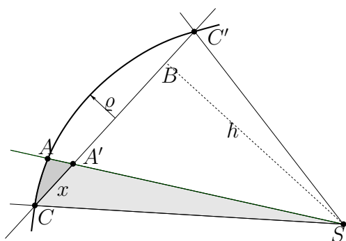
Fig. 3. By applying the second Kepler's law one sees that the motion on the chord is approximately uniform (see text).
