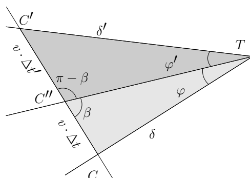
Fig. 4. Using the second observation and the uniformity of the motion on the chord the distance \delta' can be calculated as a function of \delta .
