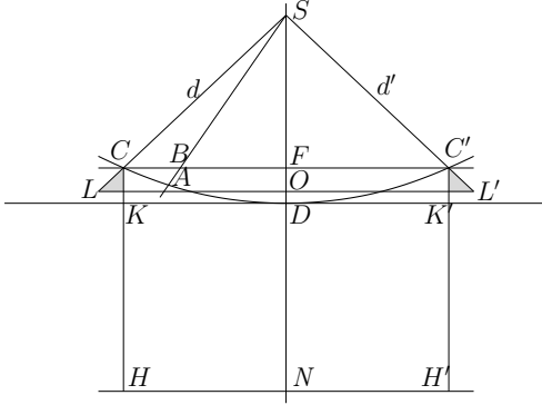
Fig. 5. Illustrating the search for an average velocity in the simplest case. S is the focus (the Sun), the straight line HH' is the directrix and D is the vertex (the perihelion). The positions C, C' are chosen to be symmetric with respect to the axis of the parabola, which makes the geometric considerations simpler. Thus, the tangent to the parabola in D is parallel to the chord CC' . By the properties of the parabola the equalities |SD| = |DN| , |SC| = |CH| and |SC'| = |C'H'| hold true. The point F is the intersection of the chord CC' with the radius SD , and the point O is such that |DF| = 3|DO| . Recalling that the area between the parabola CDC' and the straight line KDK' is \frac{1}{3} of the area of the rectangle CC'K'K we get that the area of the triangle LSL' differs from the area of the sector CDC'S of parabola only by the two small grey triangles with vertices in L, L' , which may be neglected if |DF| is small.
