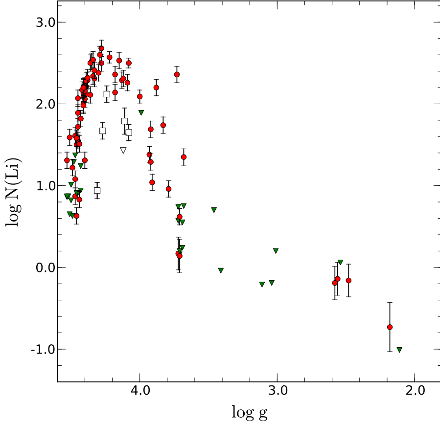
Fig. 1. Lithium abundances as a function of gravity. Downward triangles represent upper limits. Open symbols represent stars whose lithium abundances do not follow the overall trend as a function of mass. Stars with A(\text{Li}) 4.1 dex are the ones with the highest lithium abundances.
