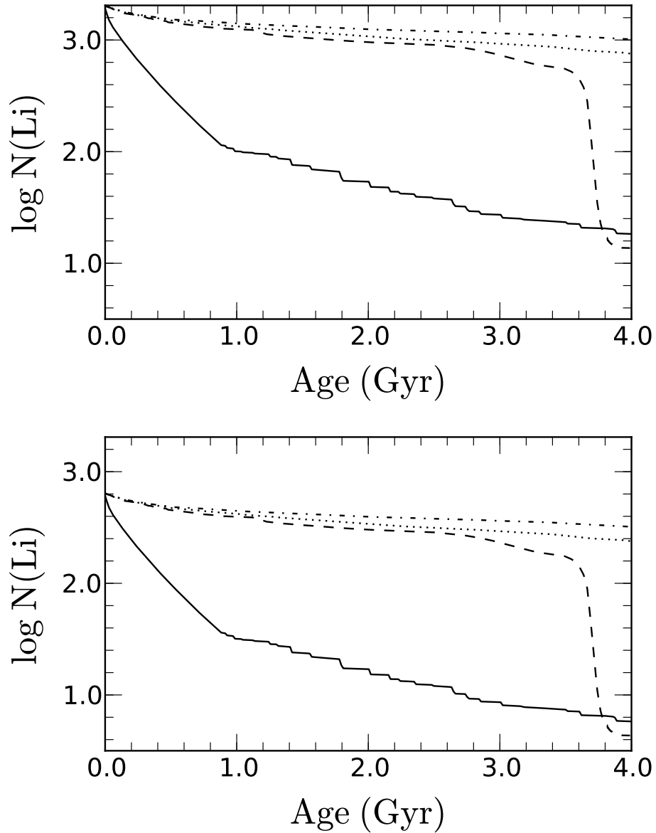
Fig. 2. Lithium abundance predicted by our models as a function of time for different masses. Upper panel: for a main sequence star with M = 1 M_{\odot} (solid line), stars of M = 1.15 M_{\odot} (dot-dashed) and 1.28 M_{\odot} (dotted) currently around the turn-off, and a more massive star of 1.33 M_{\odot} (dashed line) that is already a giant. Lower panel: same plot, but after a -0.45 dex shift was applied (as in Fig.3).
