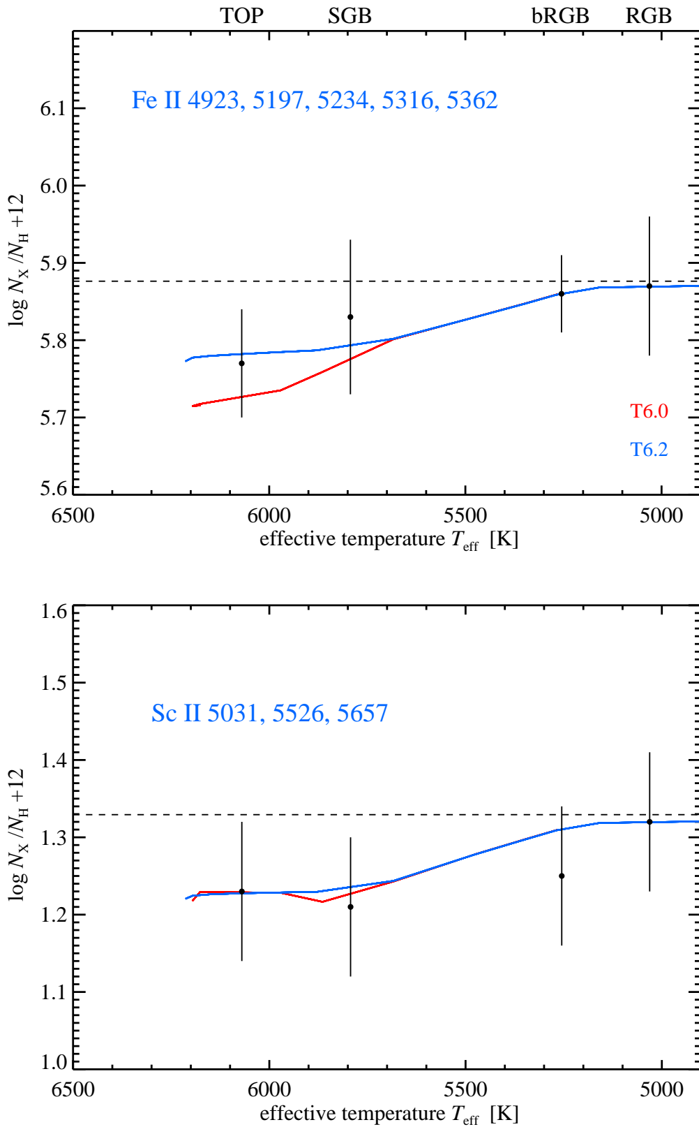
Fig. 1. Observed abundance trends for iron and scandium in NGC 6752, based on five and three ionic lines, respectively. Atomic-diffusion model predictions with NGC 6397-like (T6.0, red) and more efficient (T6.2, blue) extra mixing are overplotted (Richard, priv. comm.).
