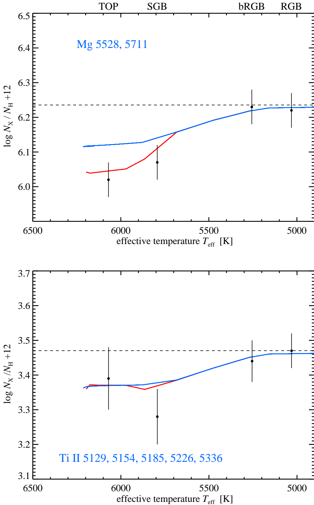
Fig. 2. Observed abundance trends for magnesium and titanium in NGC 6752, based on two high-excitation neutral and five ionic lines, respectively. Atomic-diffusion model predictions with NGC 6397-like (T6.0, red) and more efficient (T6.2, blue) extra mixing are overplotted (Richard, priv. comm.).
