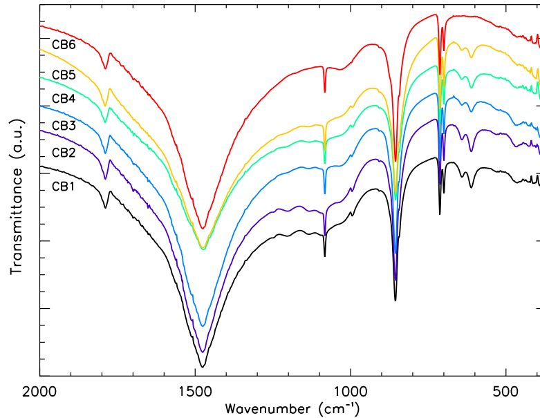
Fig. 2. Transmission spectra of the six samples (CB1 to CB6 from bottom to top) before heat processing. Spectra are arbitrarily scaled for clarity.
