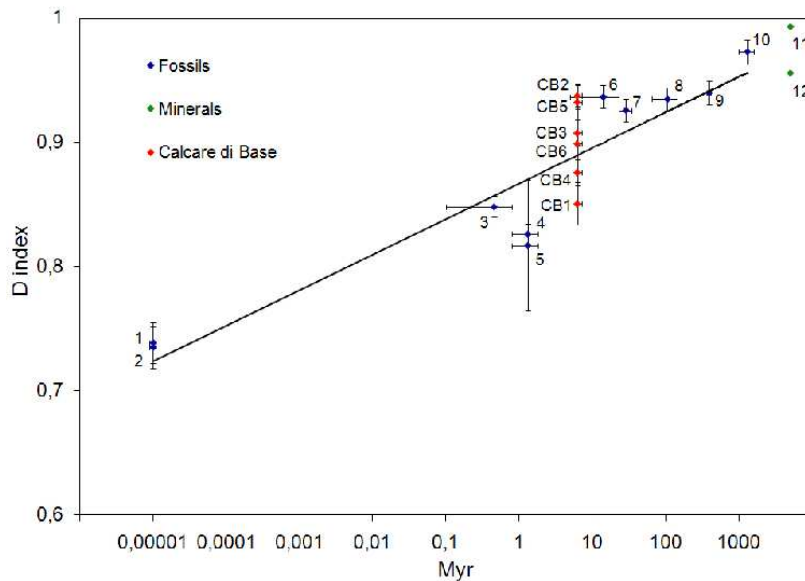
Fig. 4. Position of the six samples in the "biotic carbonate diagram". The D index for all the other samples (from #1 to #12) are those analysed by Orofino et al. (2009). The D values determined for minerals of abiogenic origin (samples #11 and #12) have to be considered outside the chronological range.
