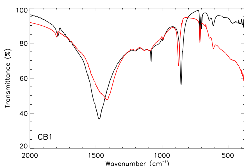
Fig. 3. IR spectra of sample CB1 before (black curve) and after (red curve) thermal processing for 3.5 hours at 485 °C.
