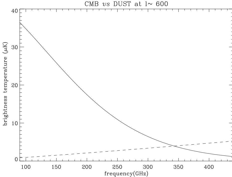
Fig. 2. The brightness temperature of CMB in \mu K (solid line) compared with the dust anisotropic emission at medium galactic latitudes (dashed line) at the multipole l \simeq 600 .
