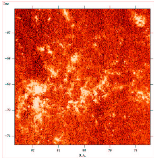
Fig. 1. MSX Spirit III infrared mosaic image of the Large Magellanic Cloud in its broad A band (centered at 8.276\mu\text{m} with a bandwidth between 6.8\mu\text{m} and 10.8\mu\text{m} ).
