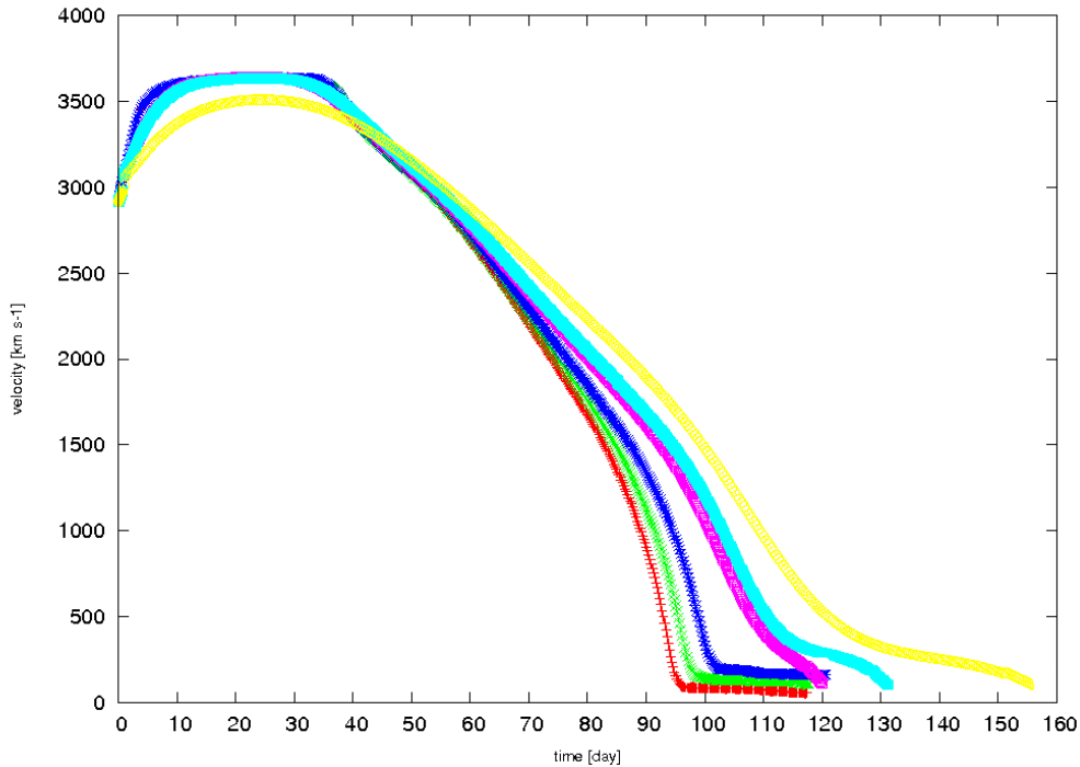
Fig. 2. Same as Figure 1, but for the evolution of the photospheric velocity.
