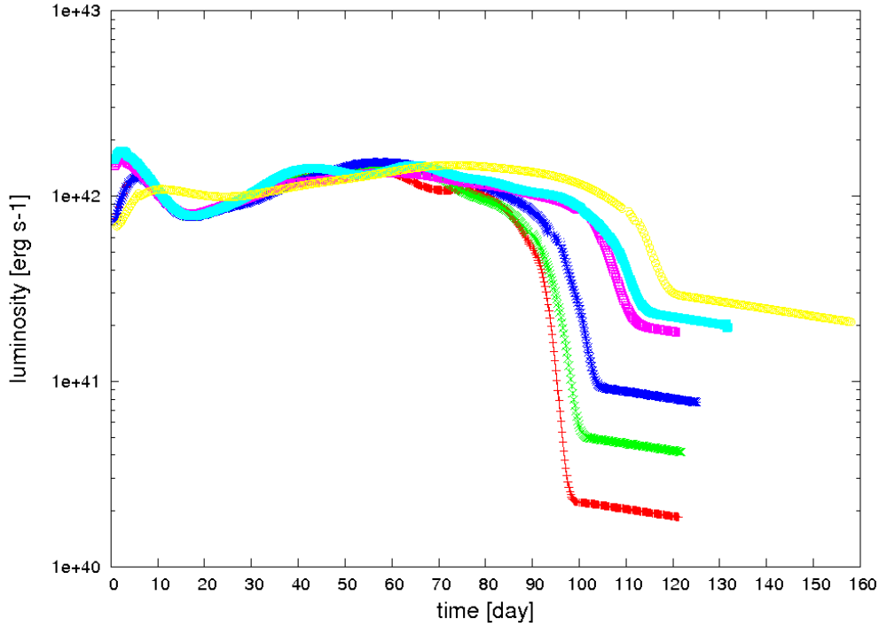
Fig. 1. Effects of varying the ^{56}\text{Ni} mass on the light curve for models having the same total mass ( 16 M_{\odot} ), initial radius ( 3 \times 10^{13} cm) and total (kinetic plus thermal) energy ( 1 \text{ FOE} \equiv 10^{51} ergs). The tracks correspond to ^{56}\text{Ni} masses equal to 0.005 M_{\odot} (red line), 0.010 M_{\odot} (green line), 0.020 M_{\odot} (blue line), 0.045 M_{\odot} (purple line), 0.055 M_{\odot} (cyan line), and 0.070 M_{\odot} (yellow line).
