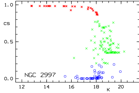
Fig. 2. The class_star classifier, cs, as a function of apparent K -band magnitude for all sources detected by SExtractor in the NGC 2997 field. Different source groups are indicated by symbols: diffuse (open circles), compact (crosses), and star-like (asterisks).
