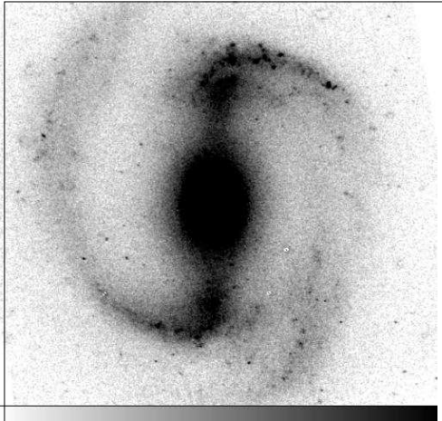
Fig. 4. The deprojected K -band image of the barred-spiral galaxy NGC 1300, which we used for our calculations in potentials with ansae type bars.
