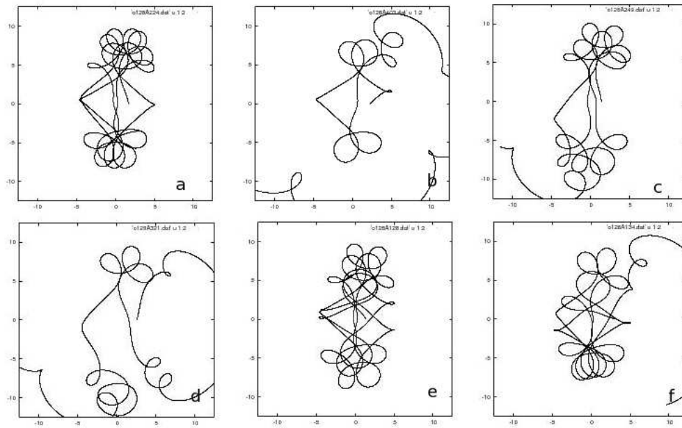
Fig. 6. Typical orbits that support barred-spiral morphologies with ansae. They support both the spirals as well as the ansae features. They are integrated for 10 bar periods.
