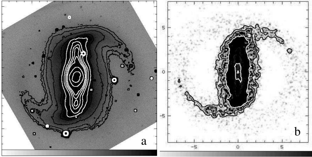
Fig. 2. (a) An R -band image of NGC 4314 showing the boxiness of the outer isophotes of the bar. We observe the limited azimuthal extent of the spirals. (b) A stellar response model of the Quillen et al. (1994) potential. The pattern rotates with \Omega_p = 38.23 \text{ km s}^{-1} \text{ kpc}^{-1} . The model reproduces the basic morphological features of the galaxy.
