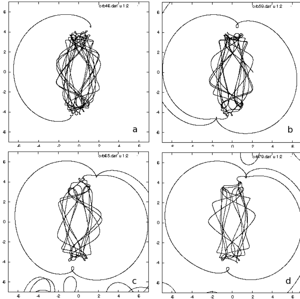
Fig. 3. Chaotic orbits of particles that support the spiral structure we observe in Fig. 2. During the time they spend in the bar region they have a rectangular-like morphology, typical of orbits at the 4:1 region of bars. They are integrated for 10 bar periods.
