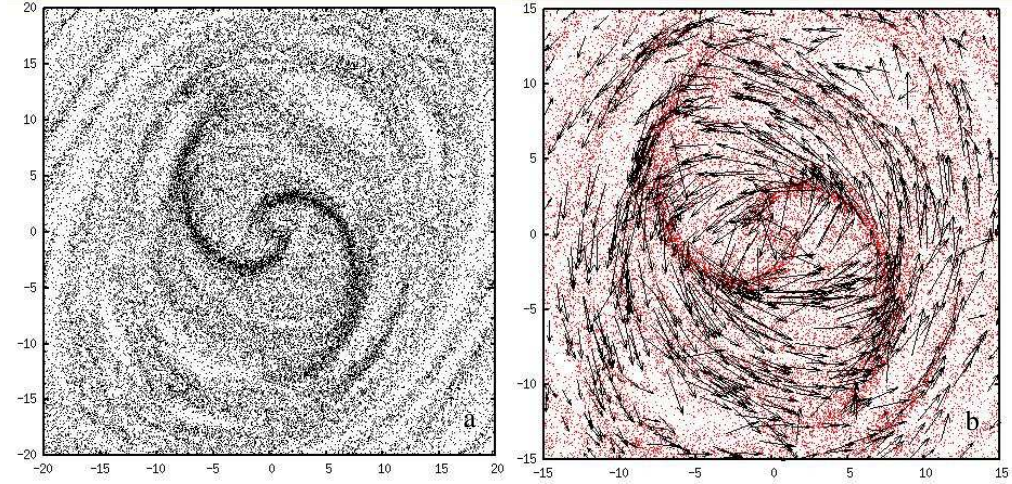
Fig. 1. The flow of stars in a time-independent stellar response model of Contopoulos & Grosbøl (1986) type. (a) The response morphology. Corotation is at \approx 24 kpc and at the end of the strong spirals, at \approx 12.5 kpc, is the inner 4:1 resonance. (b) The velocity field of the model indicated by arrows.
