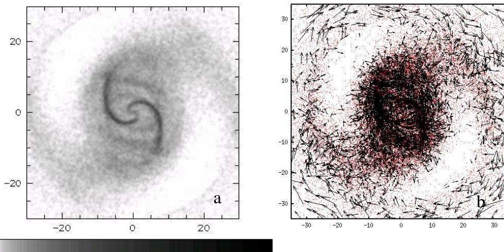
Fig. 7. A model of a double normal spiral. In (a) we observe the inner strong and the outer weak spiral. In (b) we give the velocity field with arrows, so that we can see the flow along the spirals beyond corotation.
