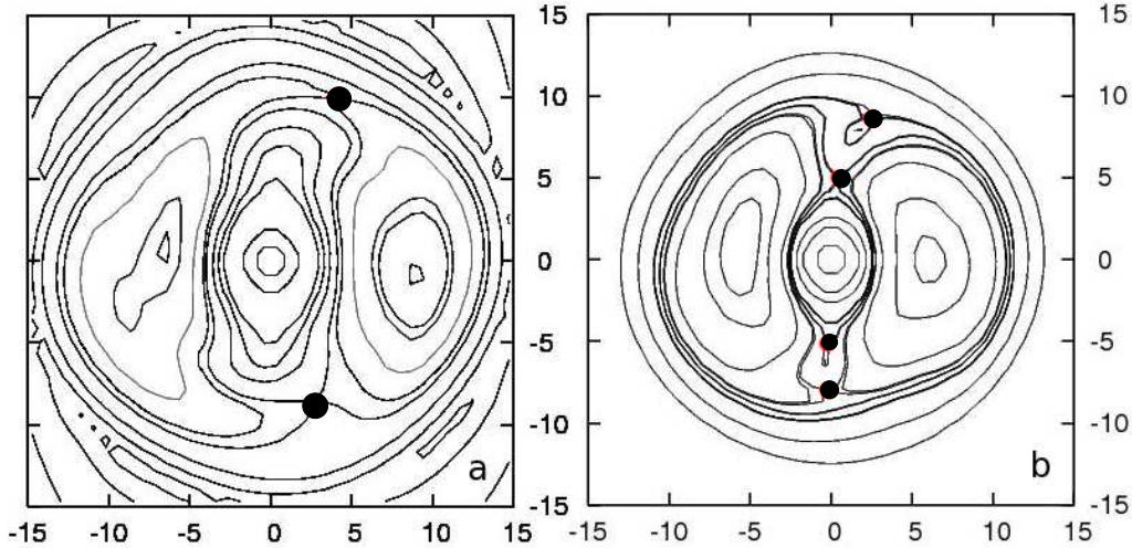
Fig. 5. Equipotentials of effective potentials in models for NGC 1300. In (a) \Omega_p=21 \text{ km s}^{-1} \text{ kpc}^{-1} and in (b) \Omega_p=26 \text{ km s}^{-1} \text{ kpc}^{-1} . Heavy dots indicate the unstable Lagrangian points in the two models.
