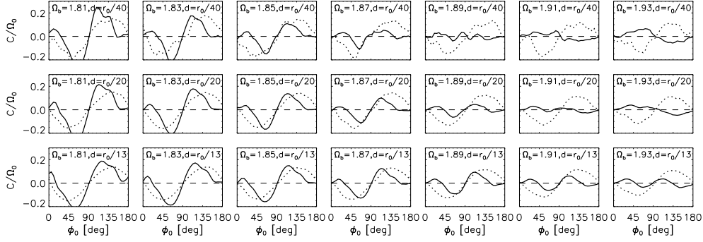
Fig. 2. Each panel shows the variation of the Oort constant C with bar angle \phi_0 , for a simulation with the parameters given in Table 1 and a particular bar pattern speed, \Omega_b , and a mean sample depth, \bar{d} . Solid and dotted lines correspond to cold- and hot-disk values, respectively. Columns from left to right, show an increasing \Omega_b in units of \Omega_0 . Note that the OLR is at \Omega_{\text{OLR}} \approx 1.7 . Different rows present results from samples with different mean heliocentric distance, \bar{d} . Good matches to the observed trend in C (vanishing value for the cold disk and a large negative for the hot one) are achieved for 20^\circ \leq \phi_0 \leq 45^\circ and 1.83 \leq \Omega_b/\Omega_0 \leq 1.91 .
