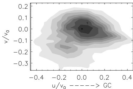
Fig. 1. Simulated u-v distribution for a bar pattern speed \Omega_b = 1.87\Omega_0 , bar angle \phi_0 = 35^\circ and a sample depth d = r_0/40 . The initial velocity dispersion is \sigma_u = 0.18v_0 and the bar strength is \epsilon_b = -0.012 . Contour levels are equally spaced. The clump identified with the Hercules stream is clearly discernible in the lower left portion of the plot. This figure is in agreement with the observed f_0(u, v) (Dehnen 1998; Fux 2001) and simulated distribution functions of Dehnen (2000) and Fux (2001).
