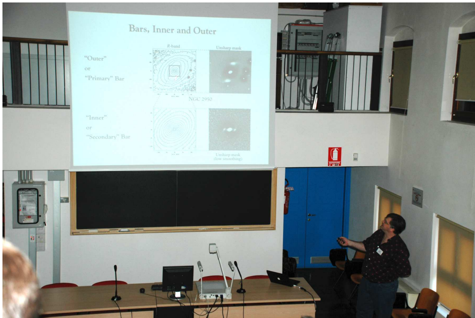
Fig. 10. Peter Erwin is dissecting NGC 2950, the prototype of double-barred galaxies, in order to separate the primary and secondary bars.
