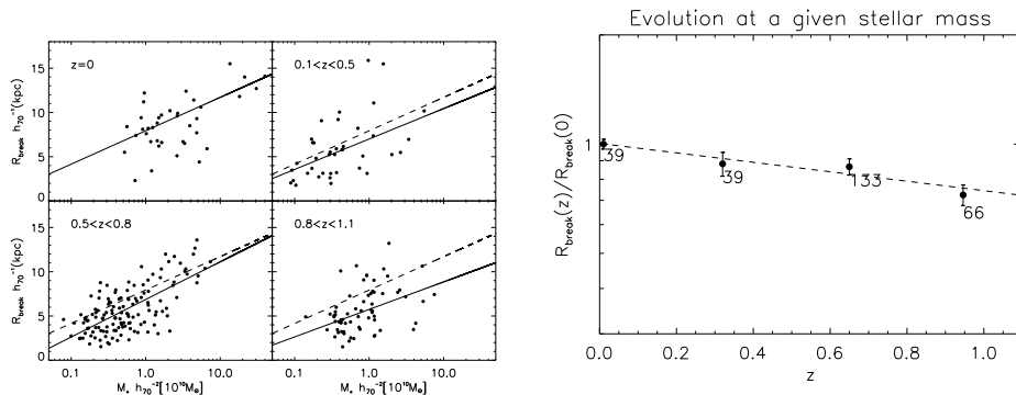
Fig. 2. Left: Break radius of ‘truncated’ galaxies as a function of stellar mass, for 4 ranges of redshift. Local data are from Pohlen & Trujillo (2006) ( g' -band results). Right: Size evolution at a given stellar mass of the break radius as a function of redshift. We have found a growth of a factor 1.3 \pm 0.1 between z = 1 and z = 0 . The numbers below each point in the right panel indicate the size of the sample.
