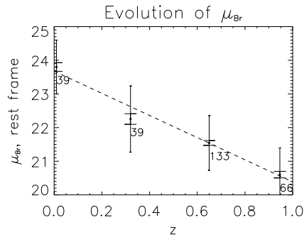
Fig. 3. Evolution of the surface brightness at the break for Type II galaxies with redshift. We show the median surface brightness at the break for the distribution of our galaxies. The larger error bars represent the standard deviation of the distributions, while the shorter ones give the error in the median values. (The numbers below each point give the size of the sample at that redshift bin.)
