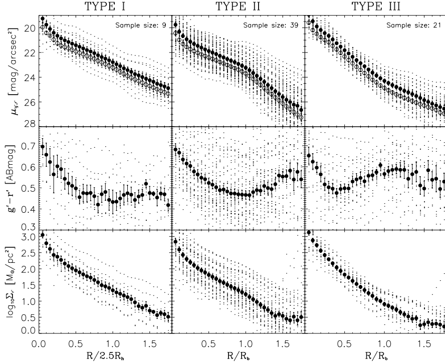
Fig. 1. Upper panels: Averaged, scaled radial surface brightness profiles of 9 Type I (pure exponential profiles), 39 Type II (truncated galaxies), and 21 Type III (antitruncated) galaxies. The filled circles correspond to the r' -band mean surface brightness, the open circles to the mean g' -band data (Pohlen & Trujillo 2006). The small dots are the individual galaxy profiles in both bands. The surface brightness is corrected for Galactic extinction. Middle panels: (g' - r') color gradients. The averaged profile of Type I reaches an asymptotic color value of \sim 0.46 mag being rather constant outwards. Type II profiles have a minimum color of 0.47 \pm 0.02 mag at the break position. The mean color profile of Type III has a redder value of about 0.57 \pm 0.02 mag at the break. Bottom panels: r' -band surface mass density profiles obtained using the color to M/L conversion of Bell et al. (2003), and using Kroupa-IMF (Kroupa 2001). Note how the significance of the break almost disappears for the Type II (truncated galaxies) case.
