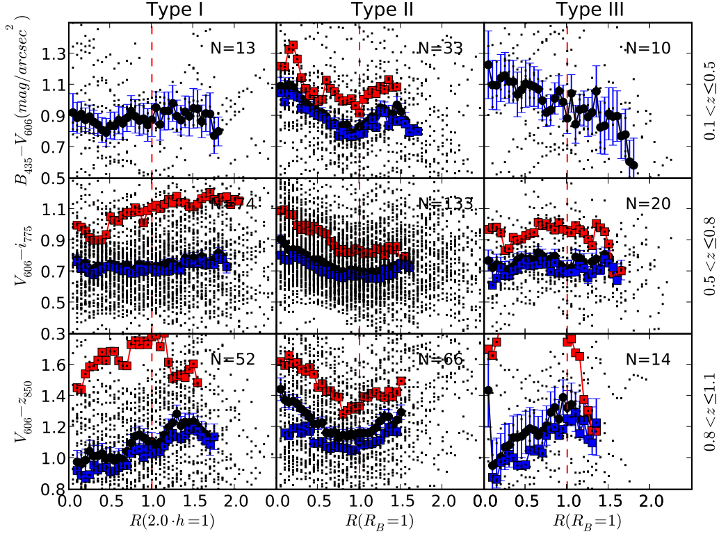
Fig. 4. Color profiles of the 415 galaxies under study in Azzollini et al. (2008a). The sample is divided in subsamples according to surface brightness profile type (I or pure exponential profiles, II or truncated galaxies, III or antitruncated), in columns, from left to right) and redshift range (low, mid, or high, in rows, from top to bottom). The colors ( B_{435} - V_{606} , V_{606} - i_{775} , V_{606} - z_{850} ) are chosen as the best proxies to the rest-frame u - g color in each redshift bin. The radii are scaled to the scale radius, R_s , whose definition depends on profile type: R_s = 2h for type I, where h is the scale-length of the disk, and it is equal to the break radius, R_s = R_B , for types II and III. Small points are individual color profiles. Large black dots are the median color profiles for each subsample, and the error bars give the error in those estimations. The red squares give the median color profile for objects with stellar mass M_\star > 10^{10} M_\odot , while the blue squares give the same for objects with M_\star \leq 10^{10} M_\odot .
