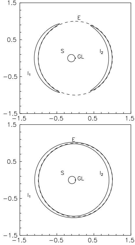
Fig. 1. Image formation for a circular source S with a radius r = 0.1 and for two different distances d between a source center and gravitational lens on the celestial sphere for d = 0.11 (top panel) and d = 0.09 (bottom panel), where I_1 and I_2 are images, E is the Einstein – Chwolson ring, GL is a position of gravitational lens on the celestial sphere.
